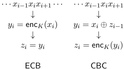
Figure: Modes of operation for block ciphers.
