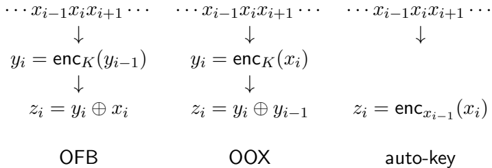
Figure: Modes of operation for block ciphers.
